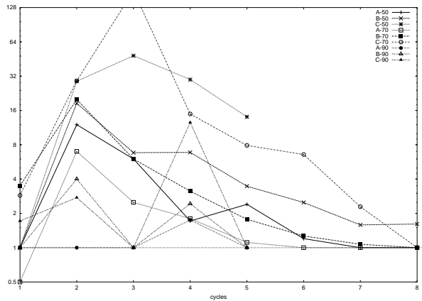
(a) Plan quality for mcs: ratio heuristic to decomp
